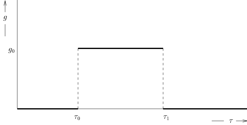
Figure 1: The linear acceleration of an observer that undergoes uniform acceleration g_0 during a period \alpha = \tau_1 - \tau_0 of its proper time. If the area under the graph exceeds a critical value given by \beta_0 \approx 1.2931 , then the convolution kernel leads to divergences.
